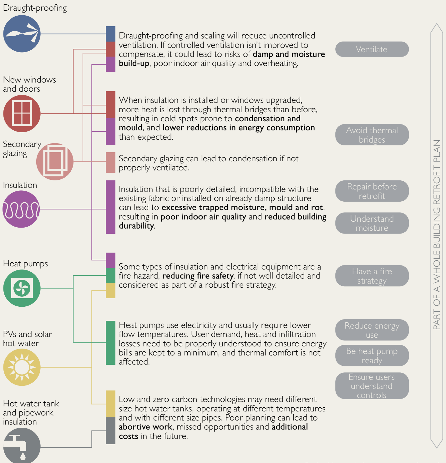
Fig. 9 Unintended consequences of retrofit adapted from Climate Emergency Retrofit Guide , LETI
